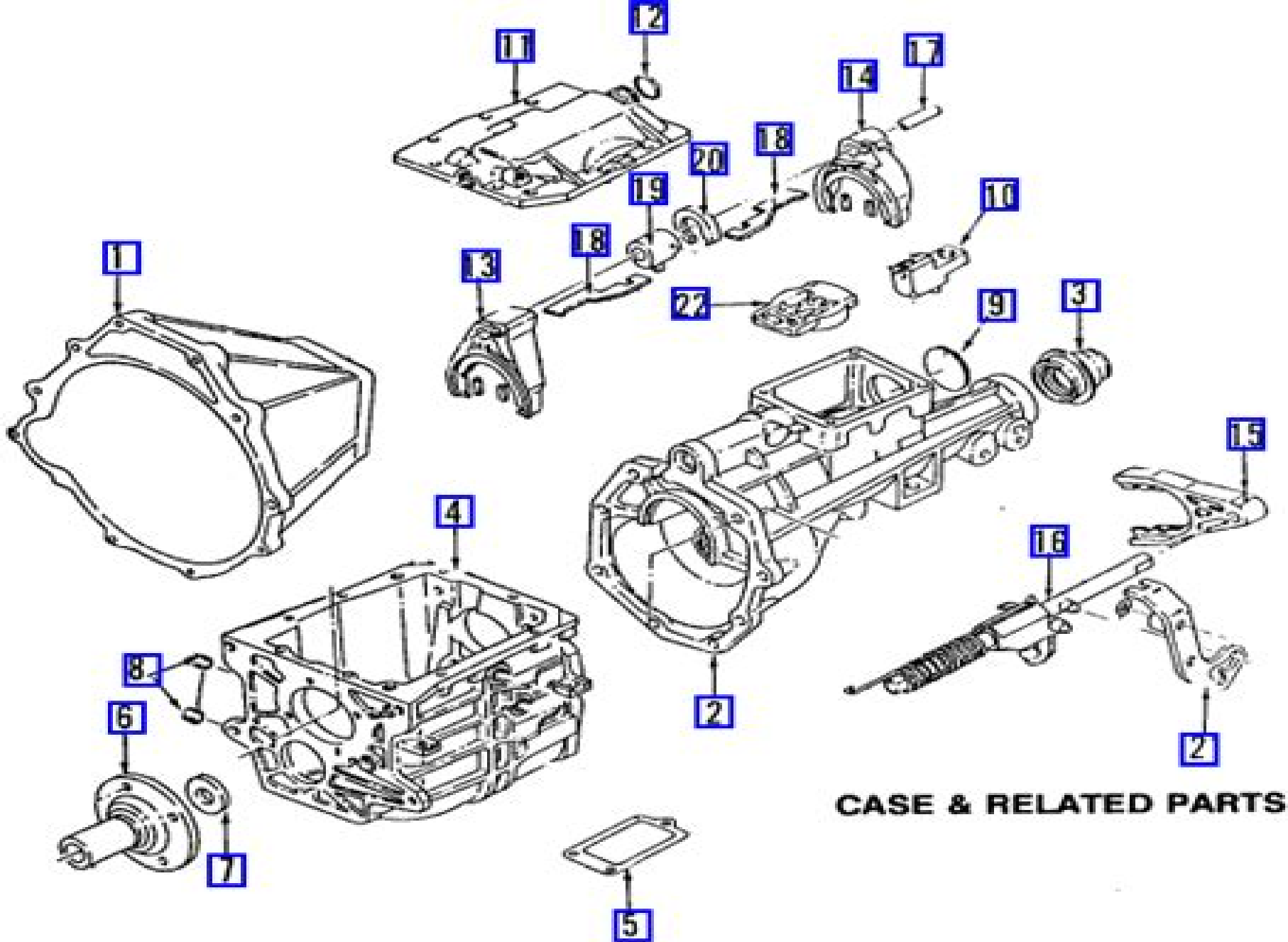
MANUAL TRANSMISSION 2WD, 3.1 LITER
