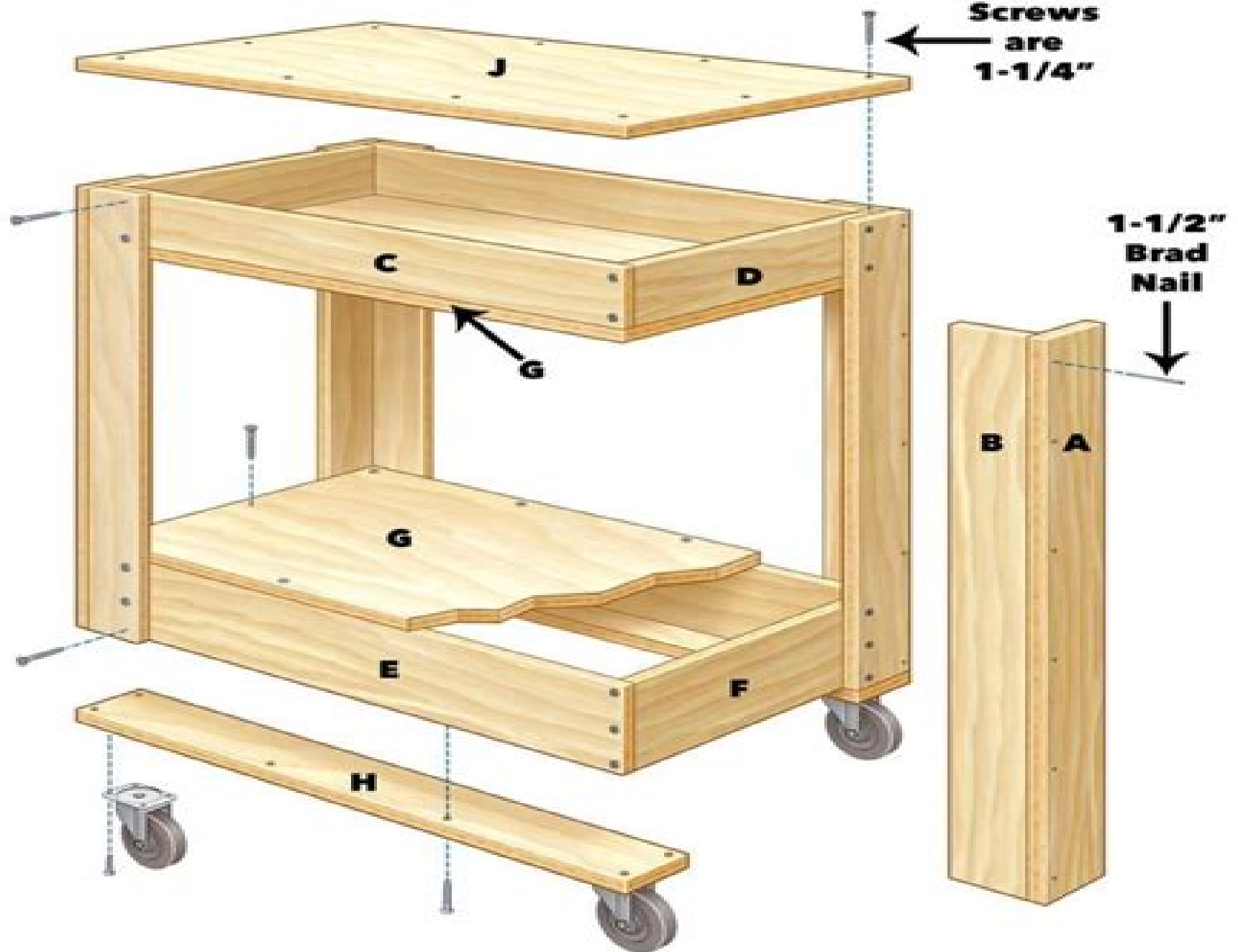
Figure A: Rolling Shop Cart
