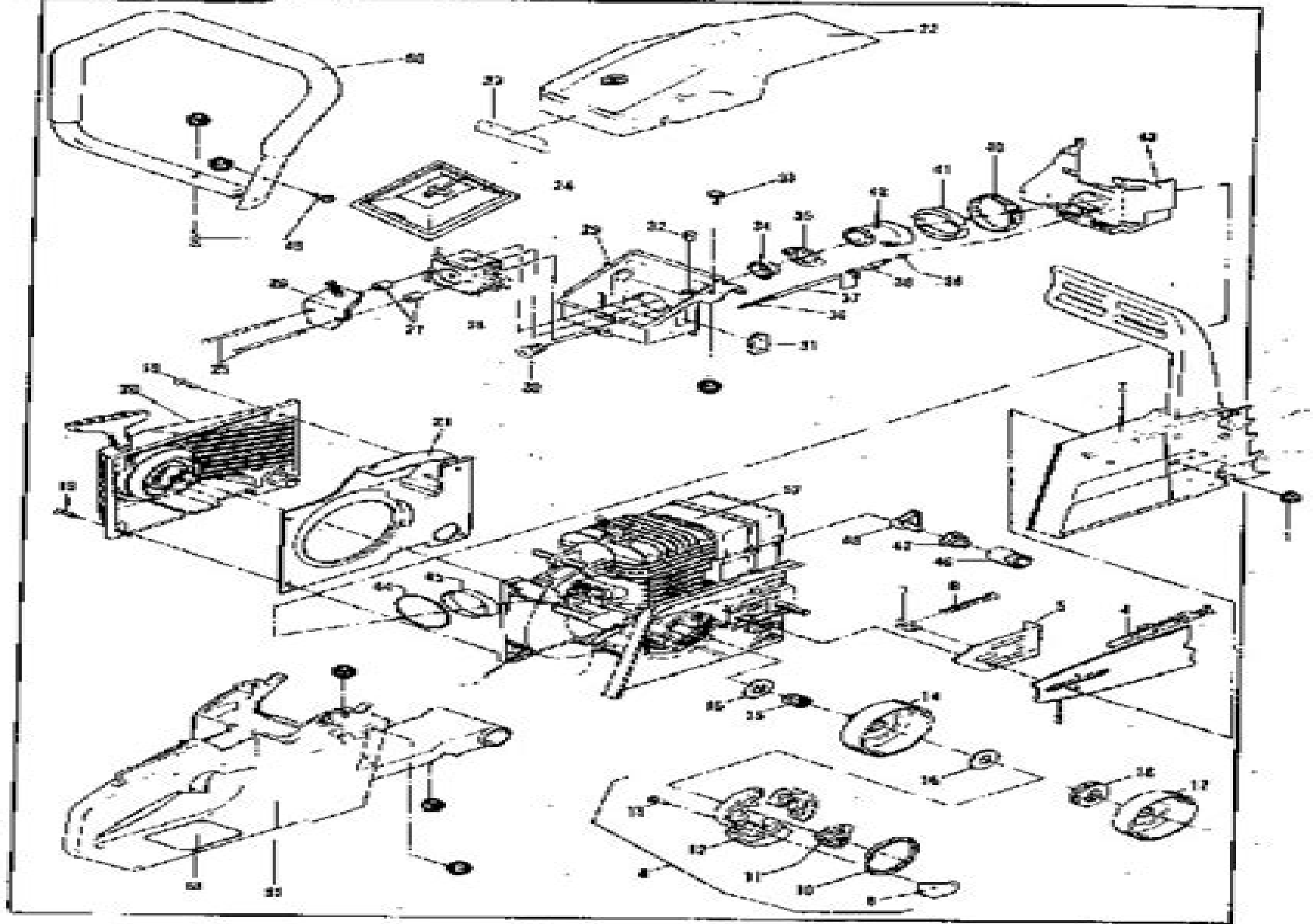
Figure 1 GENERAL ASSEMBLY
