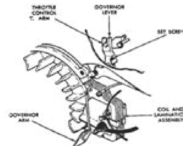
Fig. MC3-7—Typical air vane governor installation on Model 895.
