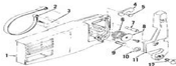
Fig. MC8-6—Exploded view of chain hooks.
