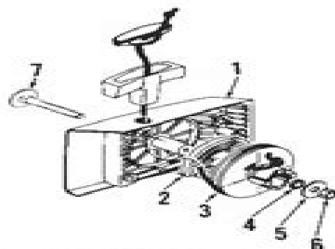
Fig. MC8-5—Exploded view of rewind starter. A screw is used in place of bolt (7) and nut (6) on some models. See text.
