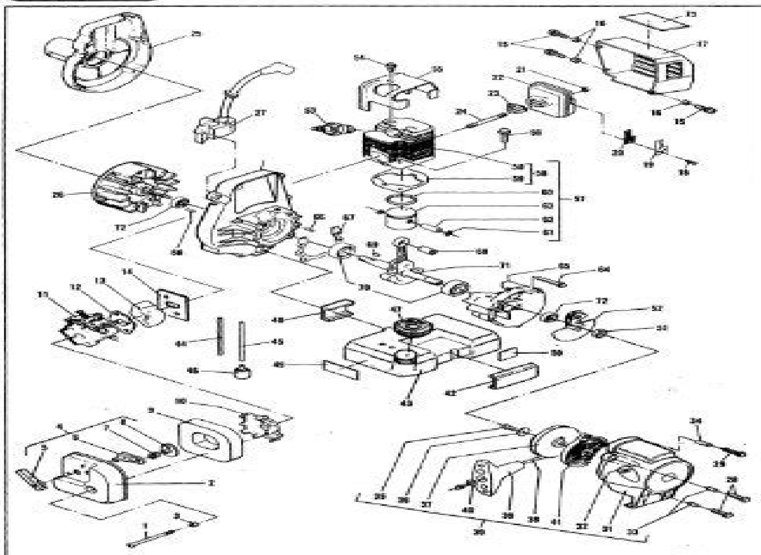
Figure 1 ENGINE ASSEMBLY
