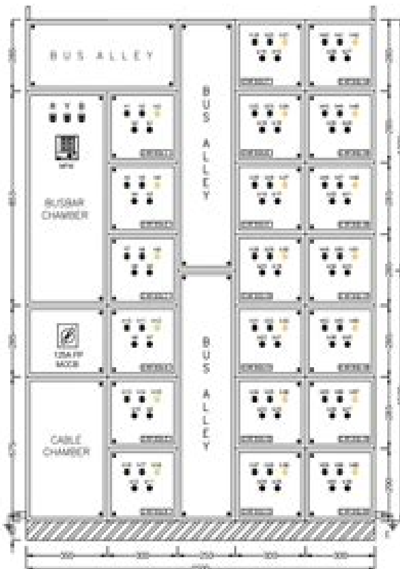
FRONT VIEW
