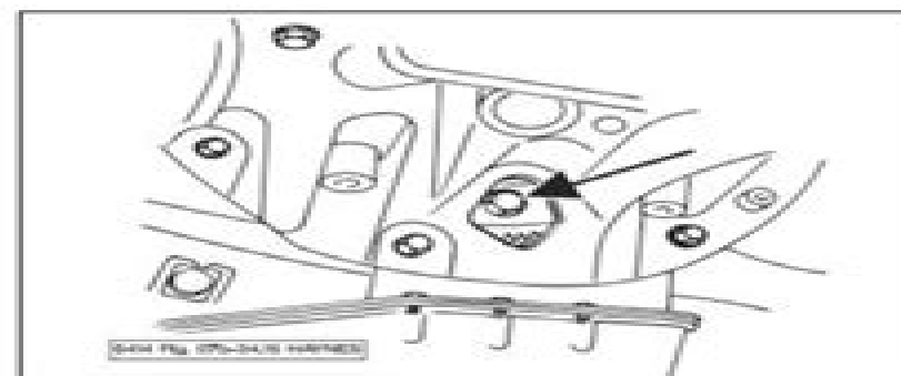
4.15 Access the torque converter mounting bolts through an opening under the engine sump
