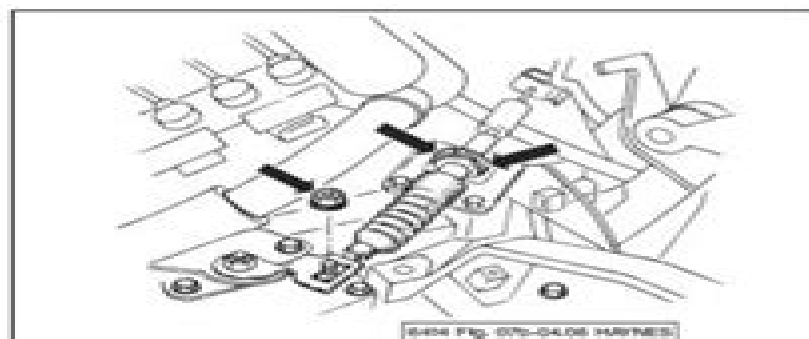
4.6 Undo the cable end fitting nut, then release the tabs and slide the outer cable upwards
