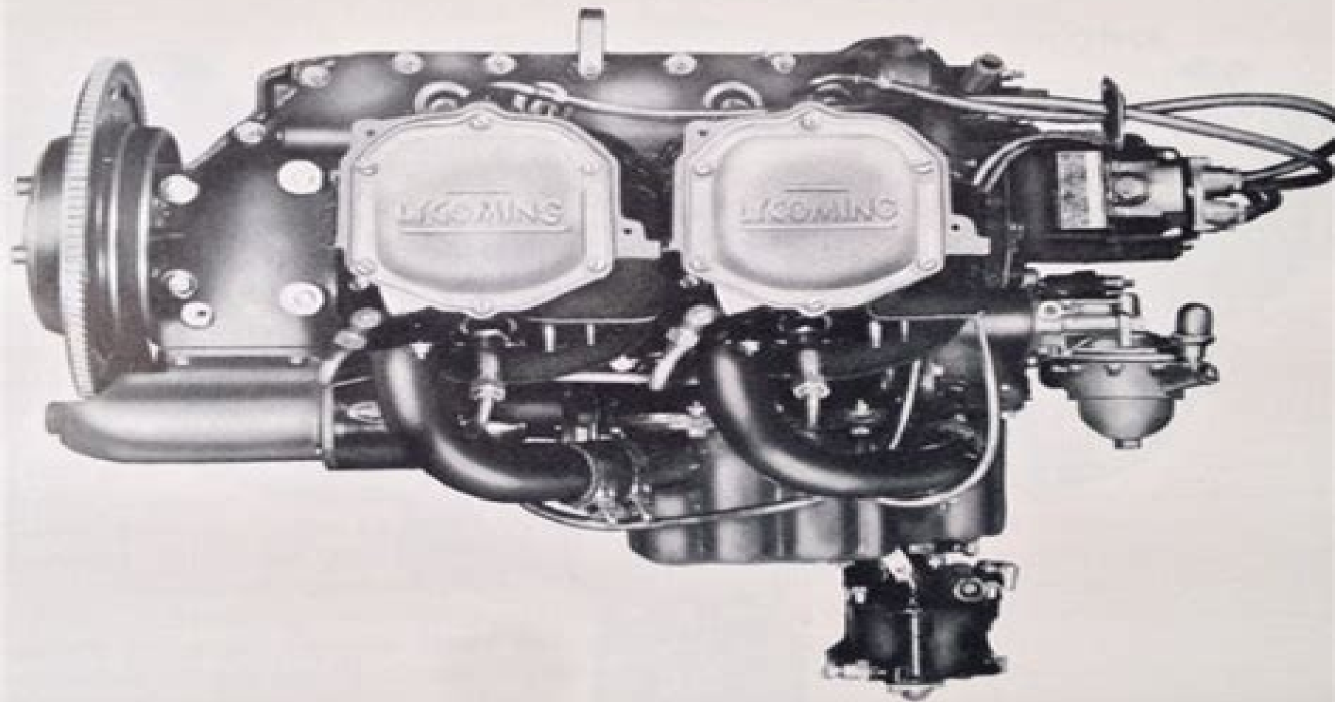
SIDE VIEW
