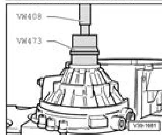
→ Fig. 1 Pressing taper roller bearing outer race out of clutch housing
