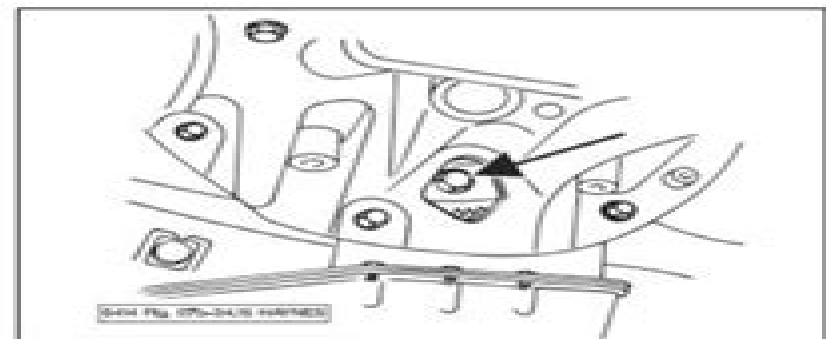
4.15 Access the torque converter mounting bolts through an opening under the engine sump
