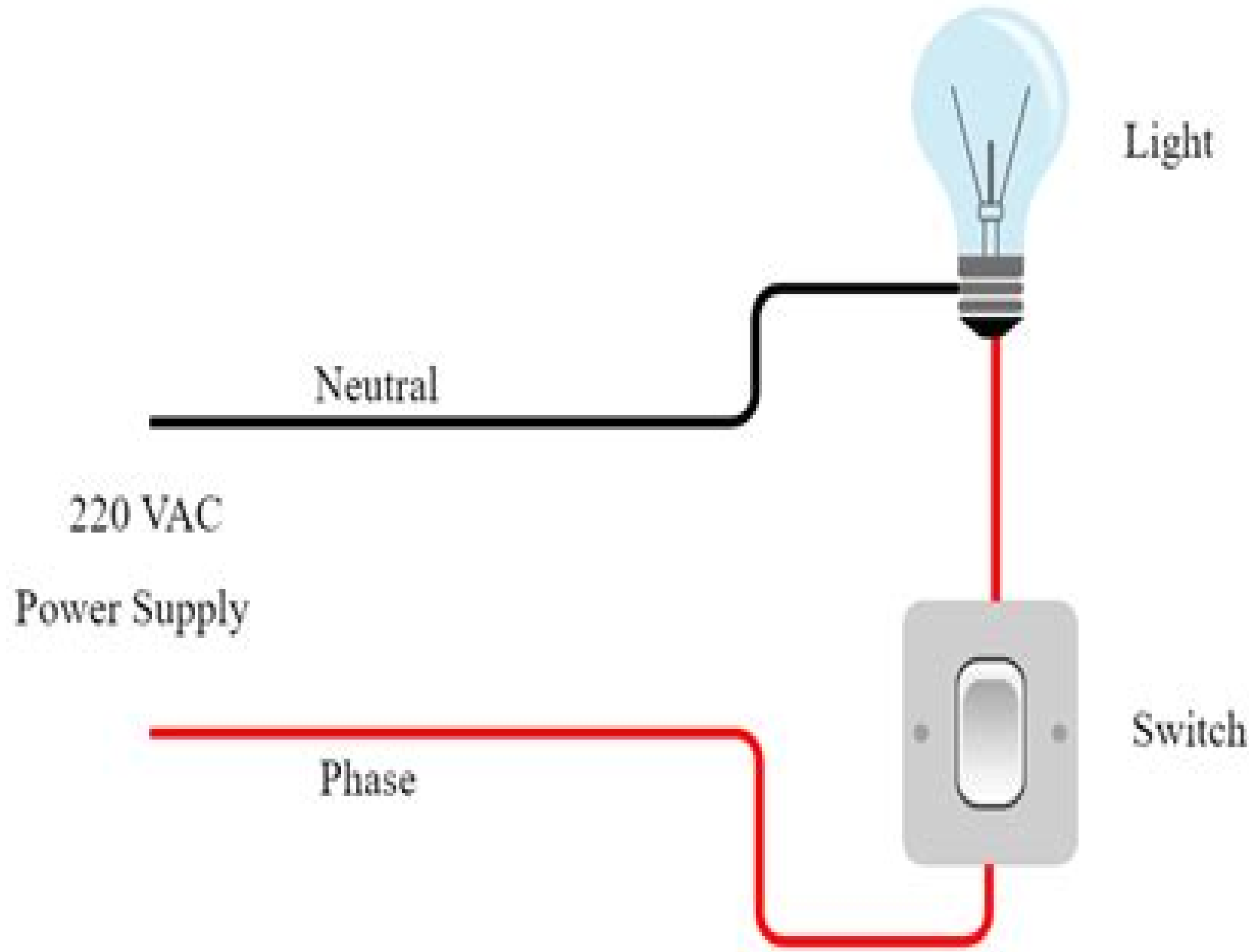
Light Switch Wiring Diagram
