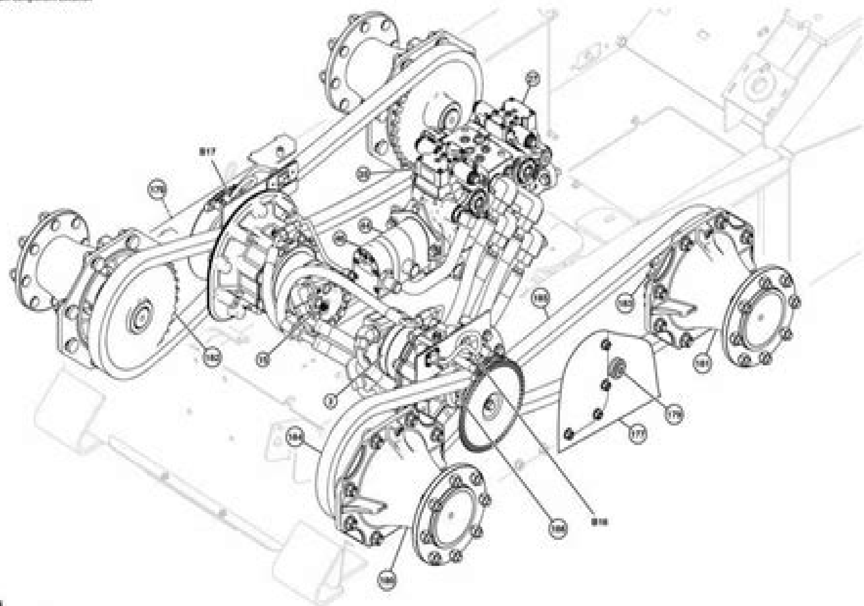
TX1003604 Power Train Component Location (single speed machine shown)
