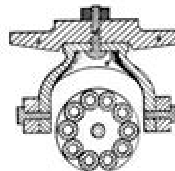
FIG. 5. SECTION THROUGH GUN BARREL, WITH AND FIRST BLOCK.
