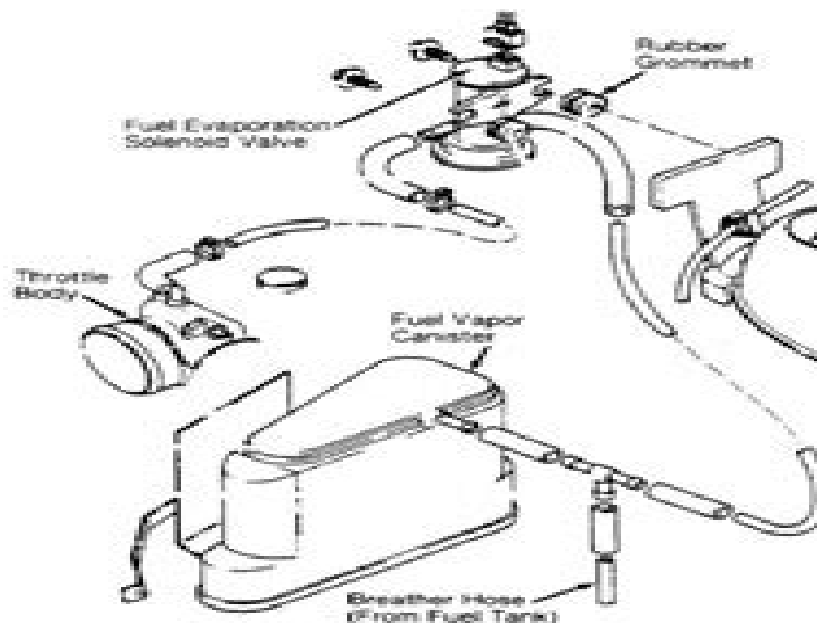
Fig. 1: Fuel Evaporation System Vacuum Diagram (EuroVan) Courtesy of Volkswagen United States, Inc.
