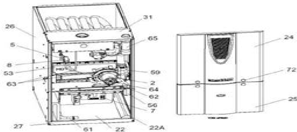
Figure 1: UPFLOW 1-STAGE NATURAL GAS FURNACES (90%)
