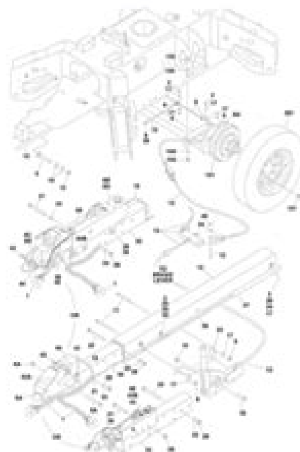
FIGURE 1-6. AXLE AND TONGUE INSTALLATION WITH HYDRAULIC BRAKES - WITH 3M BALL JOINTS AND EXPORT AND AUSTRALIAN SPEC MACHINES
