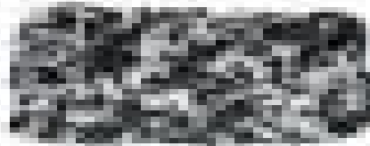
Basaltic rock (fine-grained texture)
