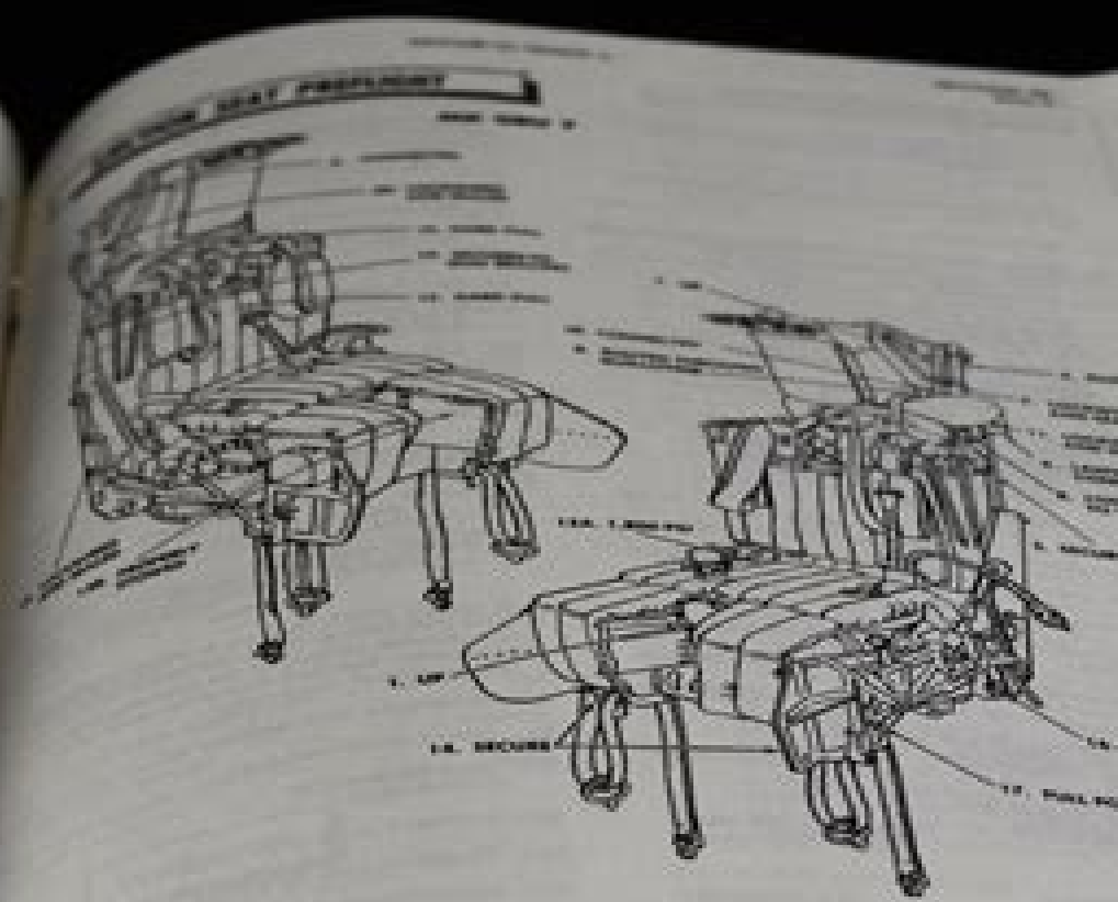
figure 2-5 Ejection Seat Preflight
