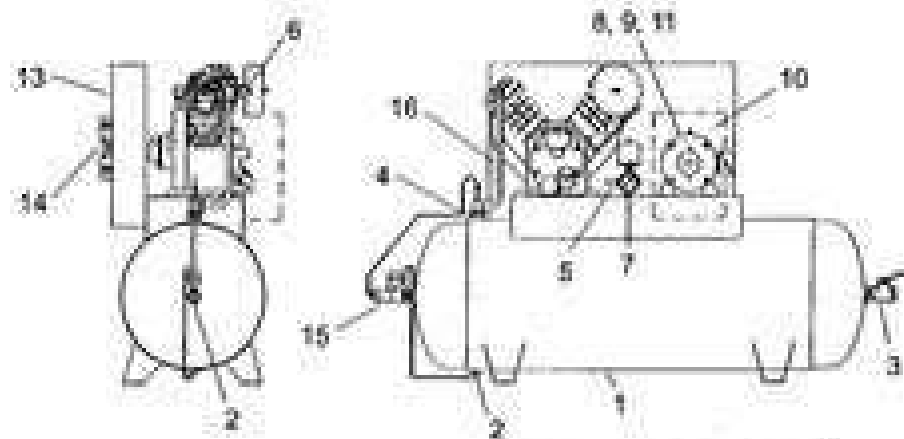
FIGURE 7. TYPICAL SIMPLEX RECEIVER MOUNTED ELECTRIC PACKAGES.
