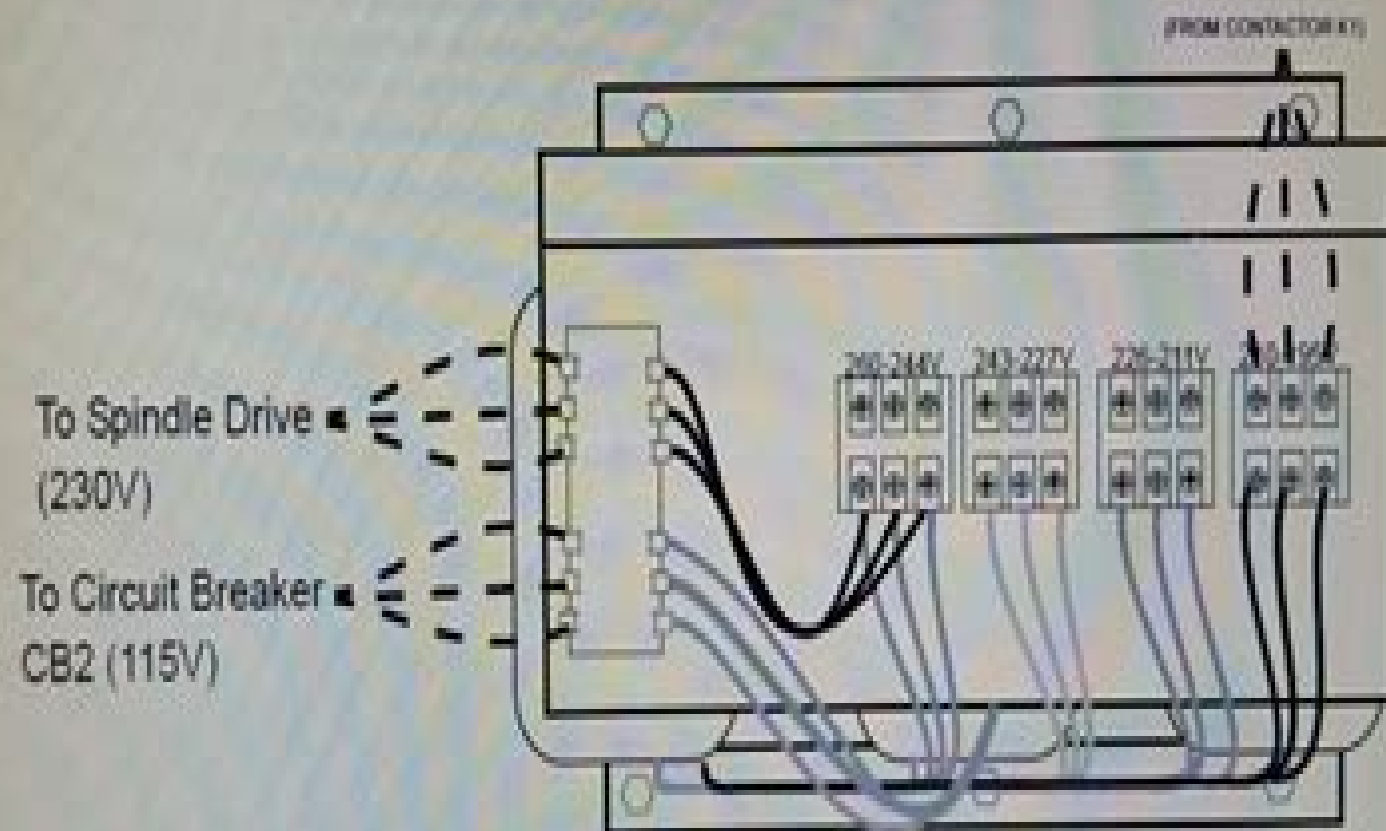
Fig. 30-1 Newer polyphase bank transformer assembly.
