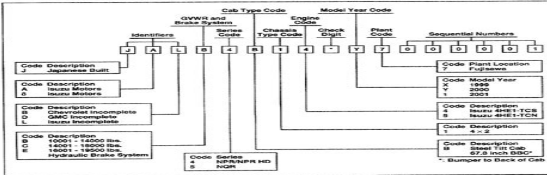
Figure 5. VIN Chart
