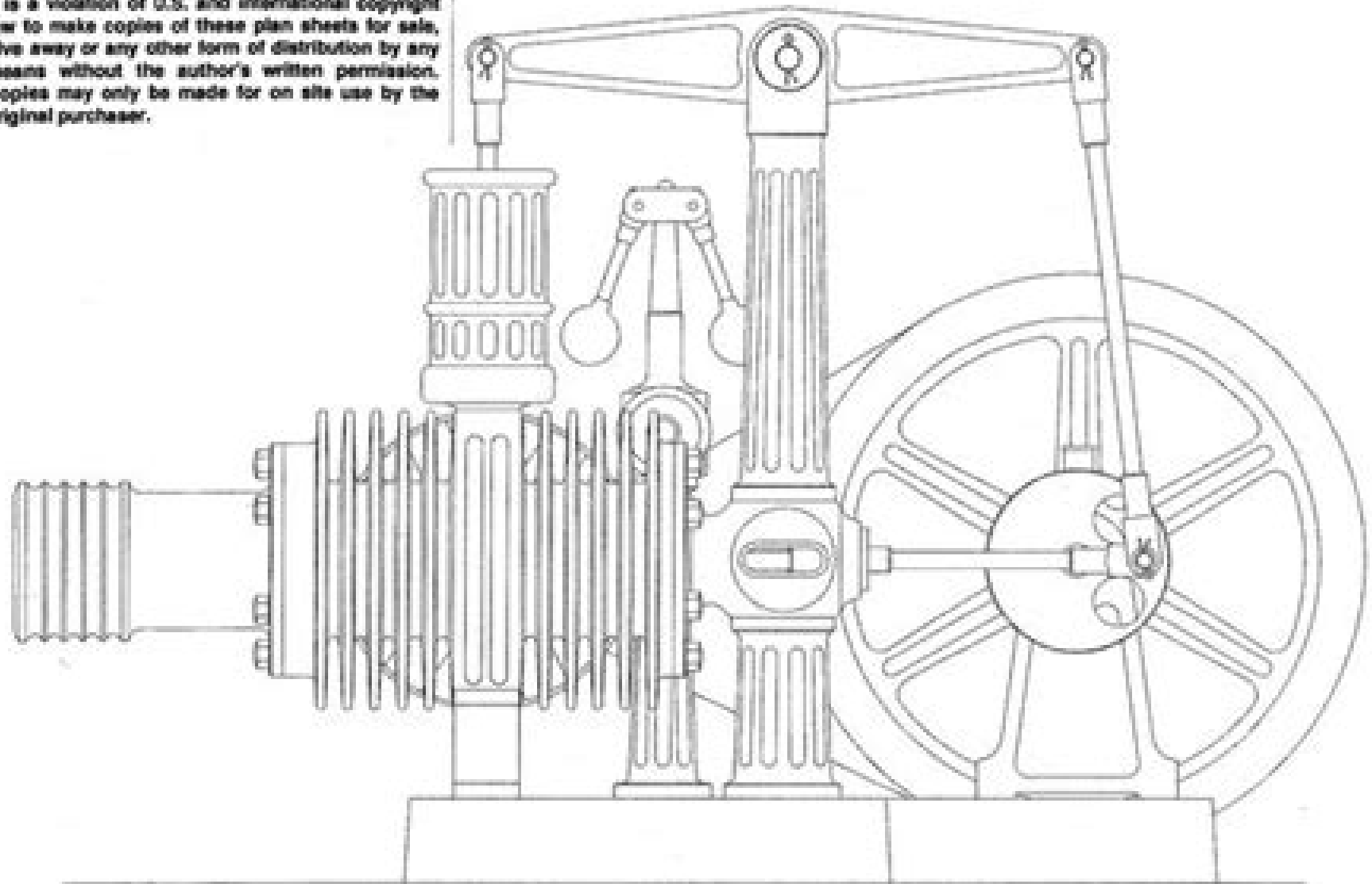
Right Side Elevation - Full Size "Beamer"
