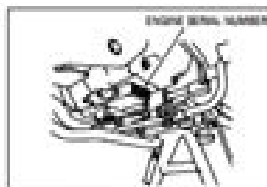
ENGINE NUMBER The engine serial number is stamped on the lower left side of the cylinder head.
