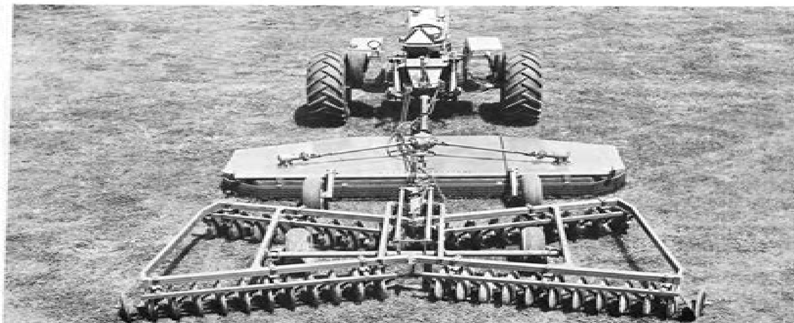
Fig. 8 - Tandem Hookup with MF 52 Disc Harrow
