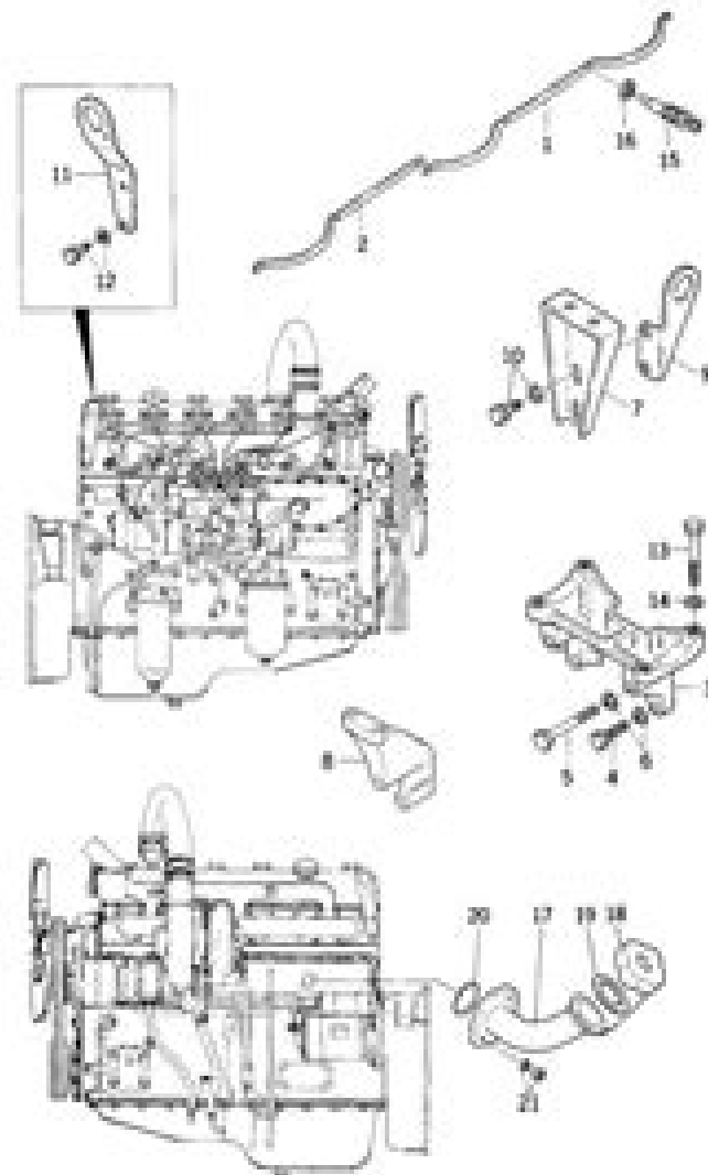
Fig. 11 CONNECTOR AND OIL FILLER
