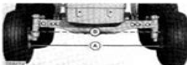
Fig. 31-Checking Toe-In
