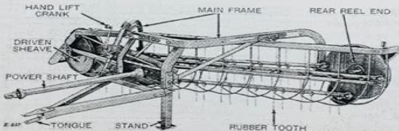
John Deere 350A Side-Delivery Rake with Semi-Integral Attachment
