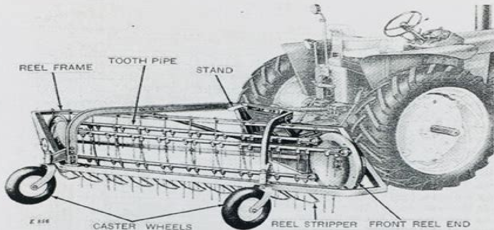
John Deere 350A 3-Point Side-Delivery Rake Mounted on a "3010" Tractor
