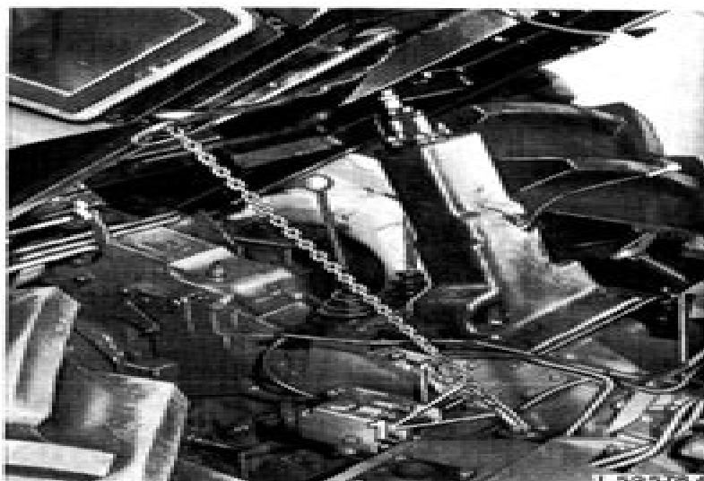
Fig. 17 — Cab Retaining Chain Installed
