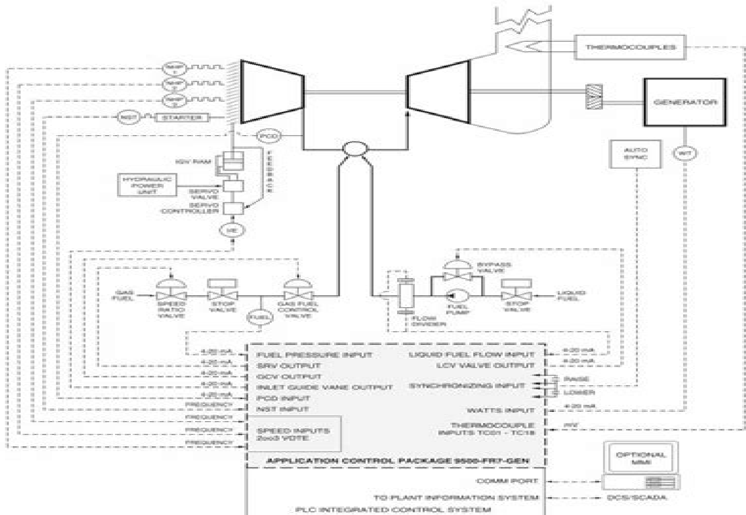
Simplified schematic showing a Petrotech GE Frame 7® gas turbine generator drive application control package integrated into an advanced PLC-based control system. Shown with dual fuel system.
