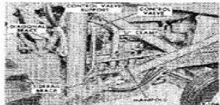
Figure 7—Loader Control Valves and Hydraulic Lines
