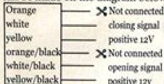
(Figure B positive trigger wiring diagram)
