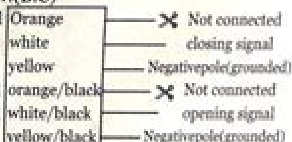
(Figure C Negative trigger wiring diagram)
