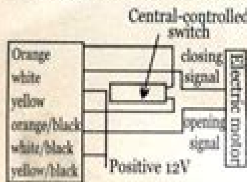
(Figure E wiring diagram for positive electric circuit installation)
