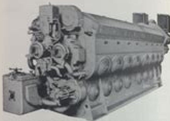
Front Three-Quarter View MGC Engine Fig. 1-2
