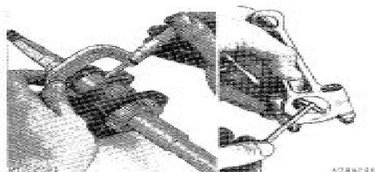
Fig. 31-Measuring Crankshaft
