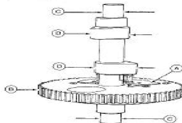
A—Compression Release Mechanism B—Camshaft Gear
