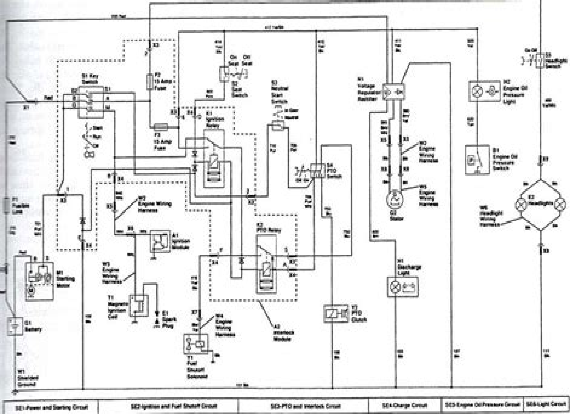
FIGURE 10: Wiring schematic and harness diagram for Model GT275
