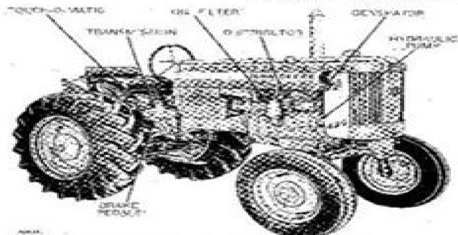
Figure 10-5-3—Parts and Assemblies Visible from Right Side of Tractor (Series "420" Standard Illustrated)
