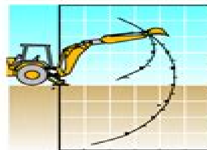
210SE BACKHOEWITH 3-FT. 6-IN. (1.07 M) EXTENDABLE DIPPERSTICK, EXTENDED
