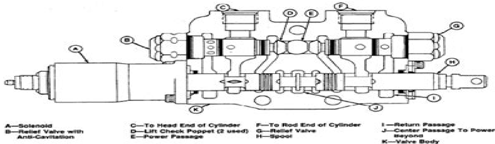
Bucket Section with Return-to-Dig
