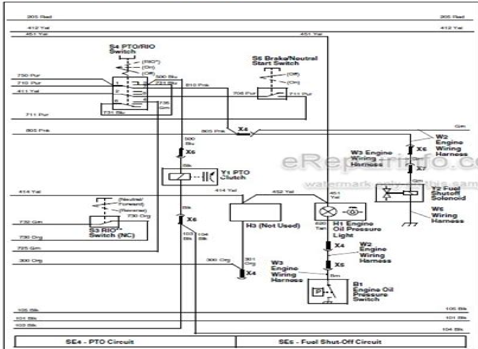
LX255 and LX266 Kohler Main Electrical Schematic (3 of 4)
