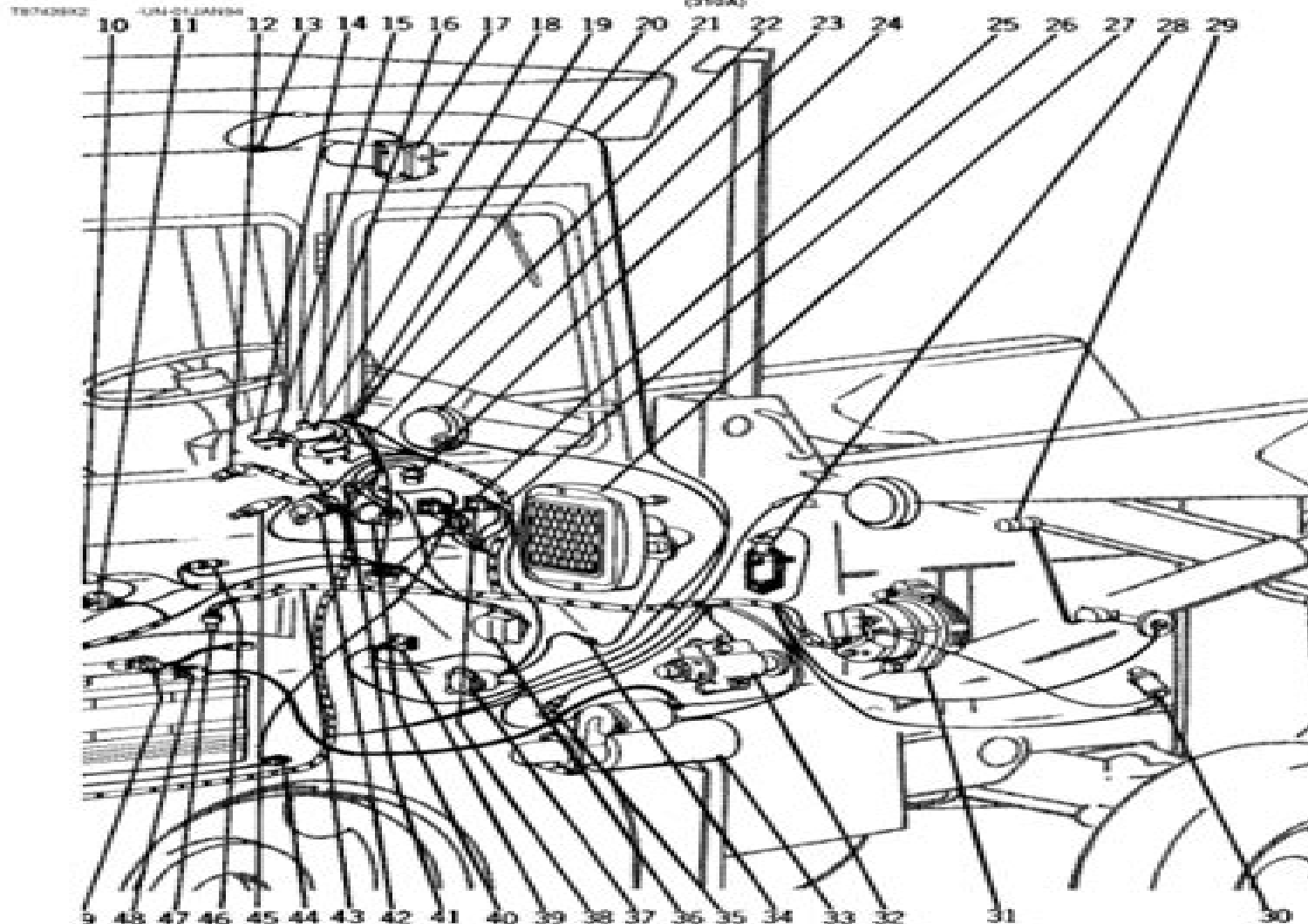
FIG. 3-ELECTRICAL SYSTEM - PART 2 (315A)
