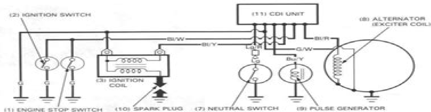
CDI SYSTEM (FOURTRAX)
