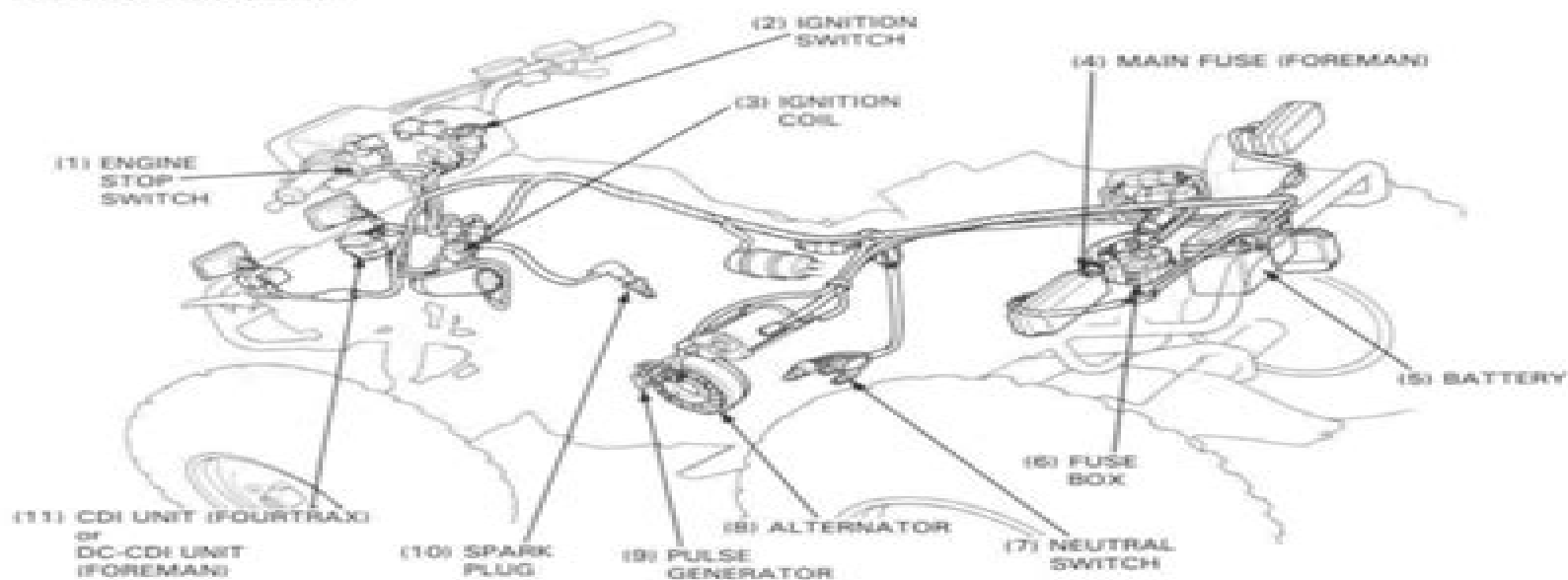
CDI SYSTEM (FOURTRAX)
