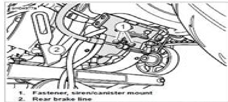
Figure 3-19. Siren/Canister Mount Plate and Brake Line
