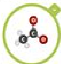
ACETATE
