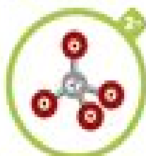
CHROMATE
