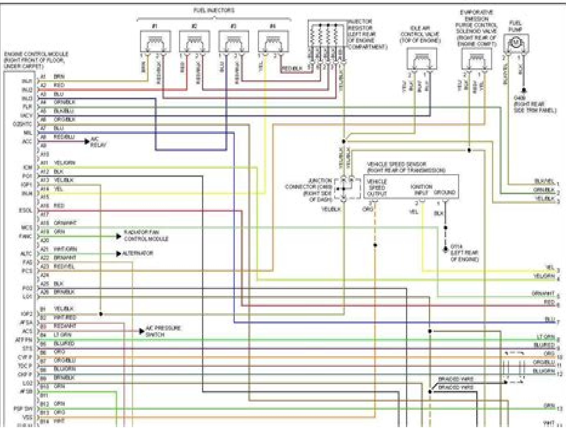
1993 Honda Odyssey LX, Pgs. 9, 10, Engine Performance Circuits (1 of 2)
