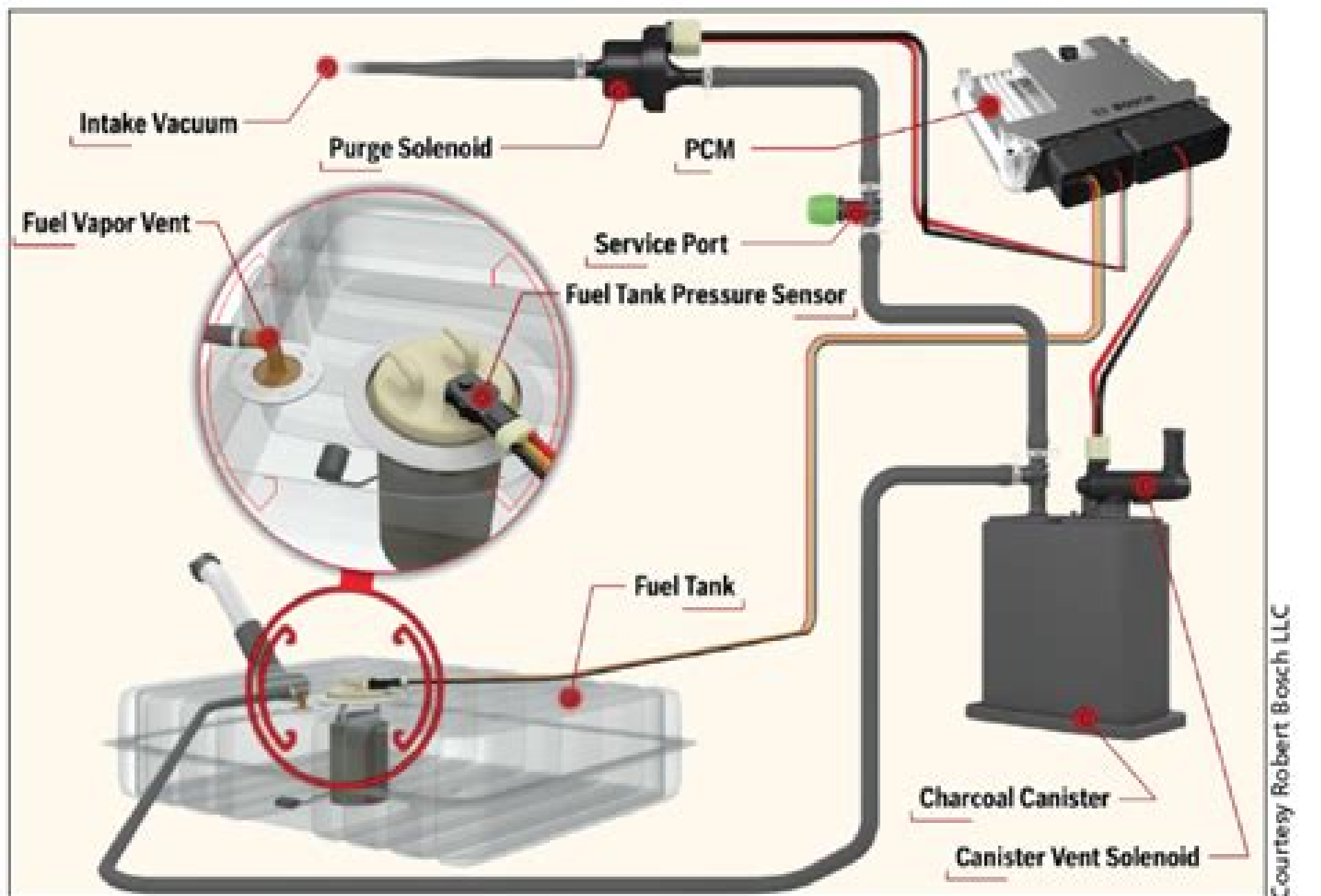
Fig. 1 This illustration shows the typical layout of components associated with Ford's vacuum-based evaporative emissions system, which has been in use for many years.
