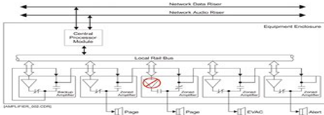
Figure 1-5: Single amplifier failure
