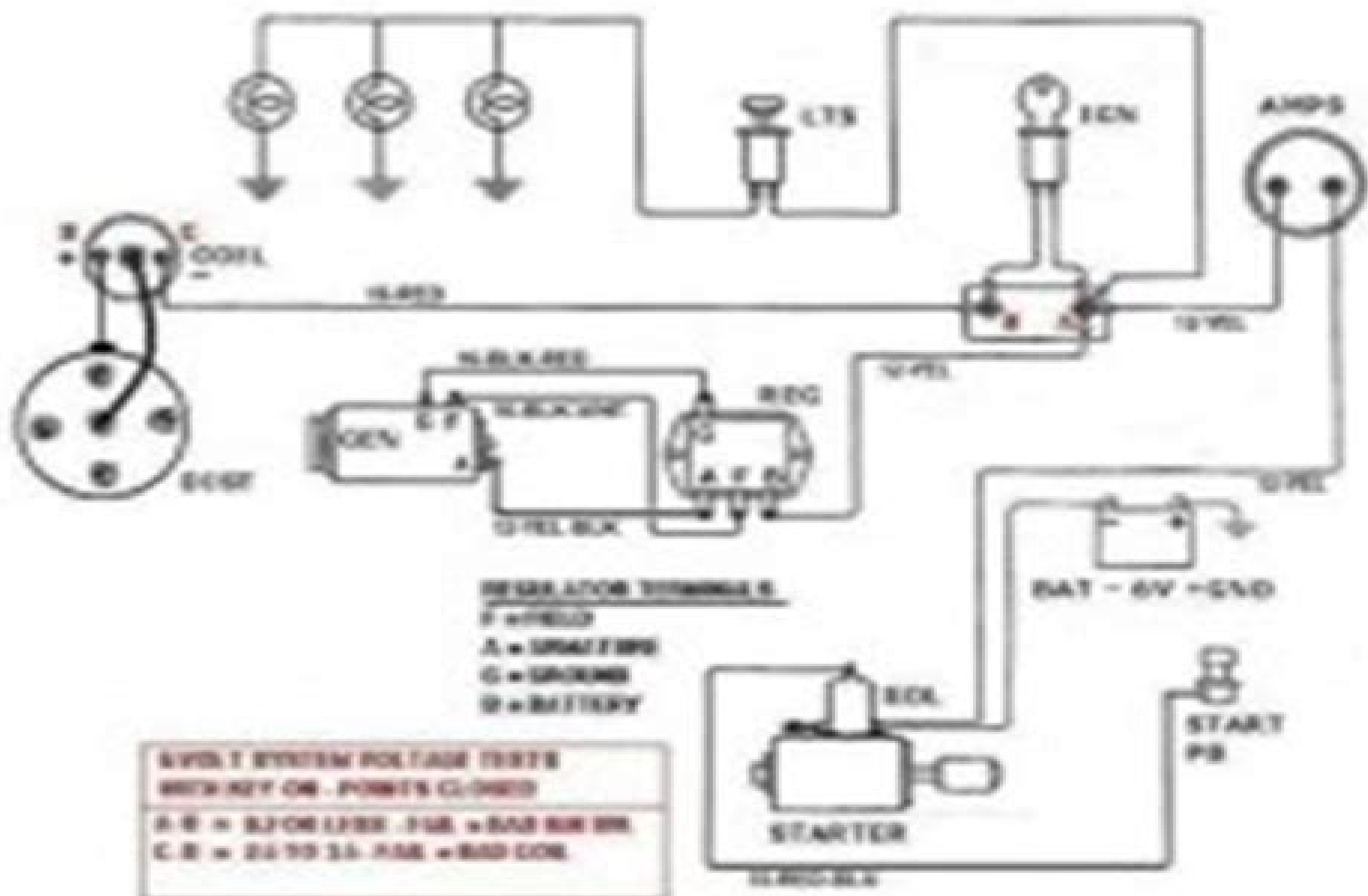
6VOLT TRACTOR WIRING - SIDE DISTRIBUTOR 1950 TO 1953 AMM. E. Laue - Free of Charge - 2008
