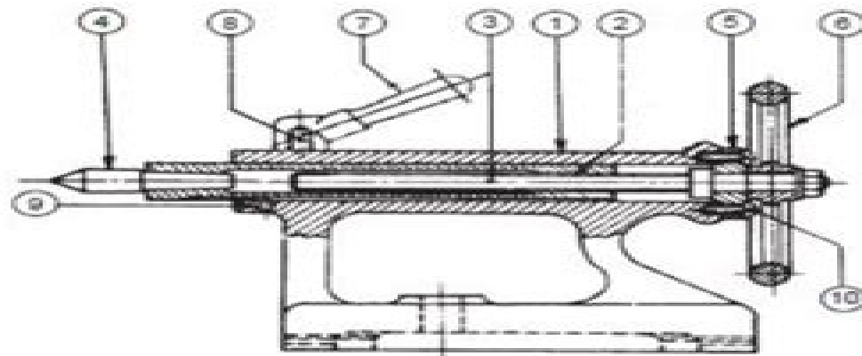
Fig. 18.18A Lathe tail-stock
