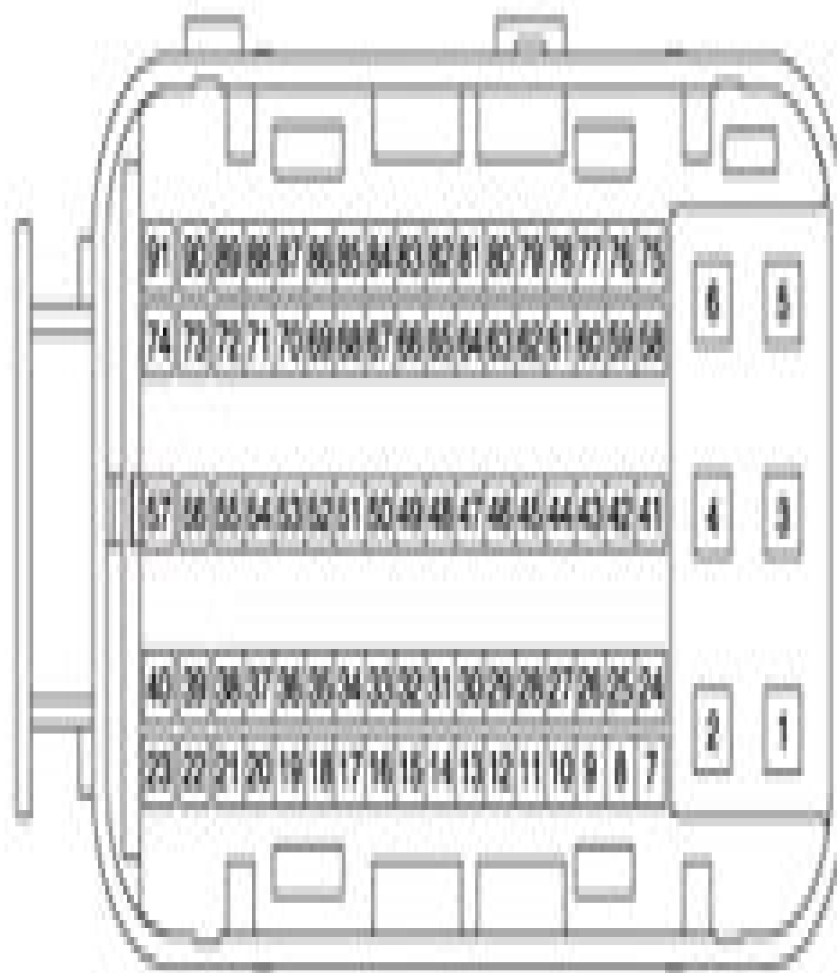
Connector (C300-B)
