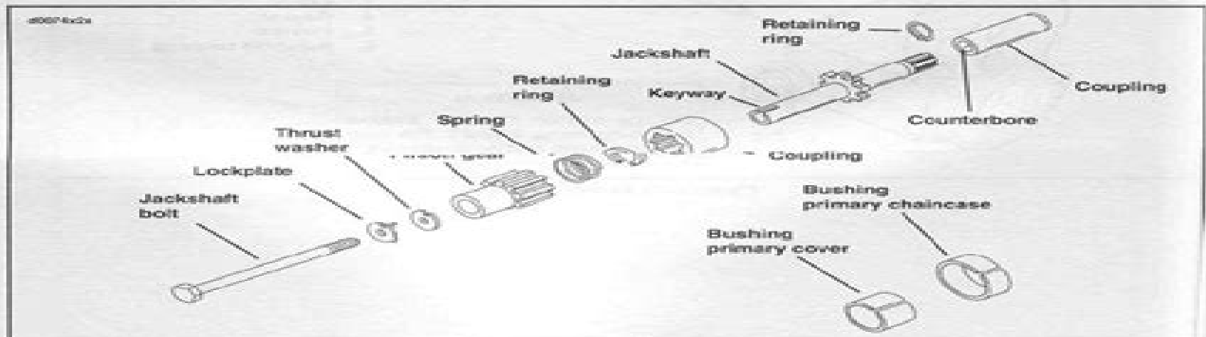
Figure 5-28. Starter Jackshaft
